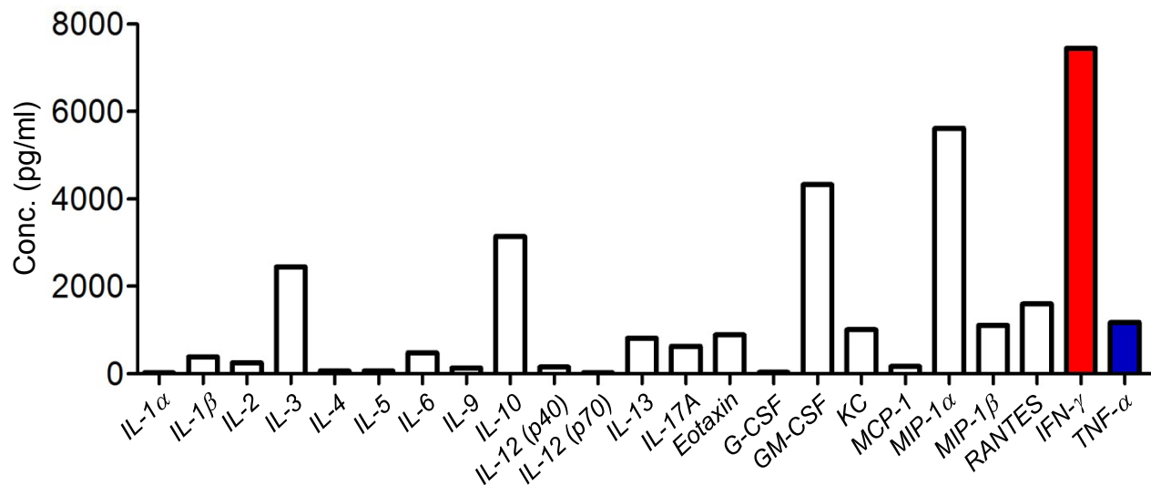
Supplementary Figure S4. Pmel-1 CTLs produce large amounts of IFN- \gamma but not TNF- \alpha in vitro. 1 \times 10^5 B16 tumor cells were cocultured with 1 \times 10^5 in vitro activated CD90.1 ^+ CTLs in a 96-well plate and 24 hours later supernatants were harvested and the concentration of cytokines measured by Mouse Bio-Plex Pro TM Assays 23-Plex Panel (Bio-Rad).
